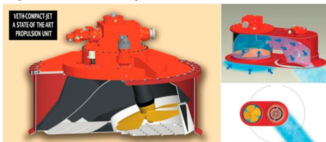
Figure 8. Flush thrusters
